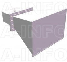
LB-975-10-C-SFSPO Standard Gain Horn Antenna 0.75-1.12GHz 10dB Gain SMA Female
